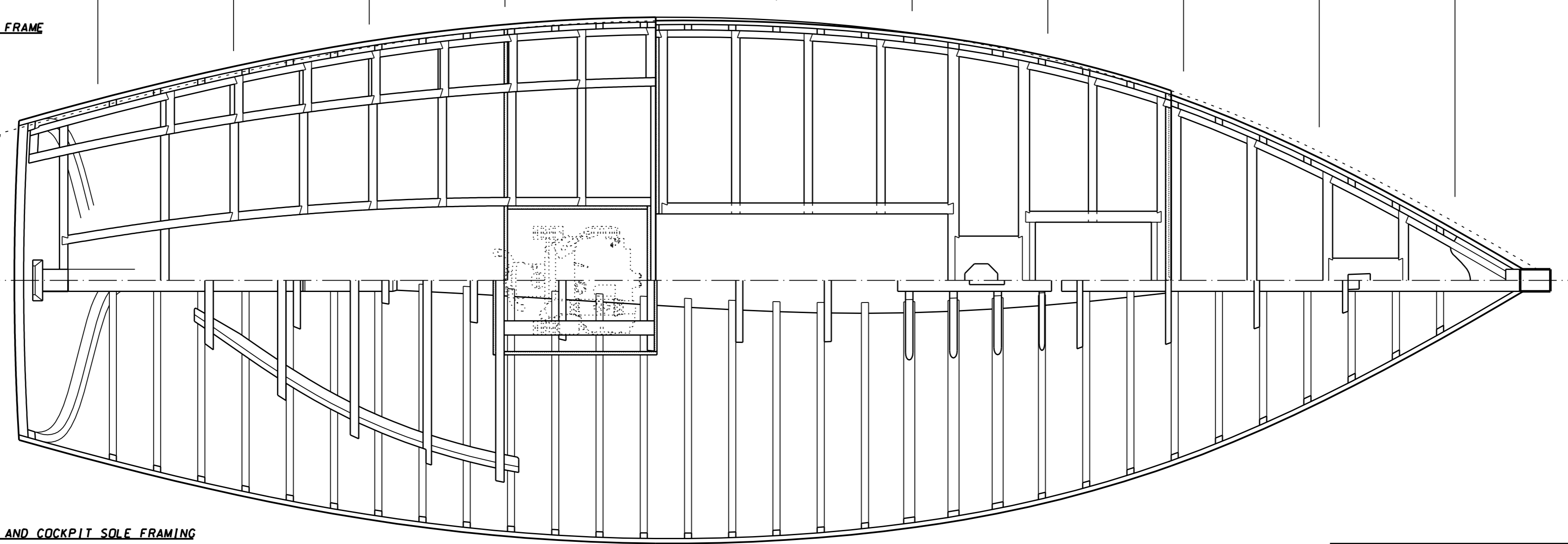
HULL AND COCKPIT SOLE FRAMING
